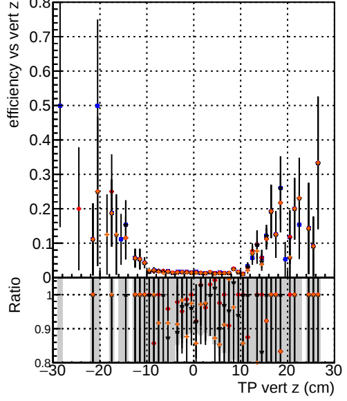
Efficiency vs vert z —●— DQM_TT_mkFit-DQM_original —●— /data2/legianni/standalone-May24/CMSSW_13_2_X_2023-06-05-1100/src/DQM_TT_mkFit-DQM_updated.0 —●— DQM_TT_mkFit-DQM_original_newwindows —●— DQM_TT_mkFit-DQM_update-mod127
