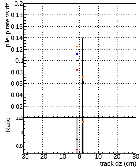
SQLM_updated=0
