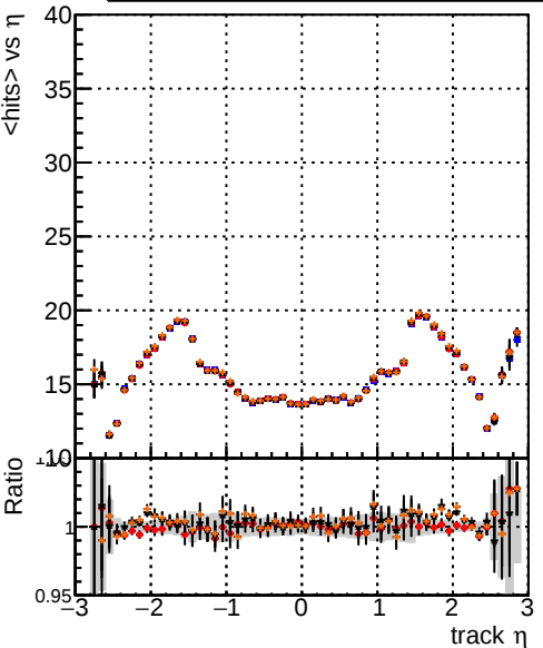
mean hits vs \eta Legend: DQM TT mkFit-DQM original, /data2/legianni/standalone-May24/CMSSW_13_2_X_2023-06-05-1100/src/DQM TT_mkFit-DQM_updated40, DQM TT mkFit-DQM original_newwindows, DQM TT mkFit-DQM update-mod127
