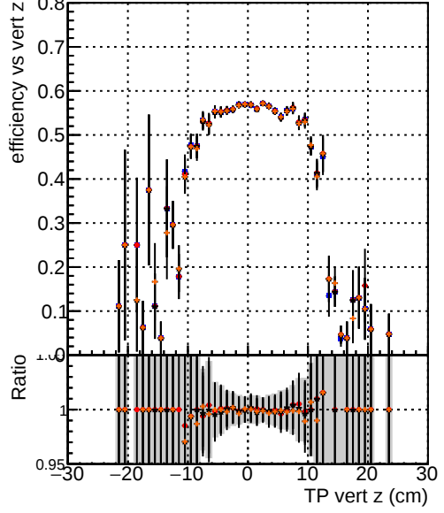
Efficiency vs. TP vert z — DQM_TT_mkFit-DQM_original — /data2/legianni/standalone-May24/CMSSW_13_2_X_2023-06-05-1100/src/DQM_TT_mkFit-DQM_updated0 — DQM_TT_mkFit-DQM_original_newwindows — DQM_TT_mkFit-DQM_update-mod127
