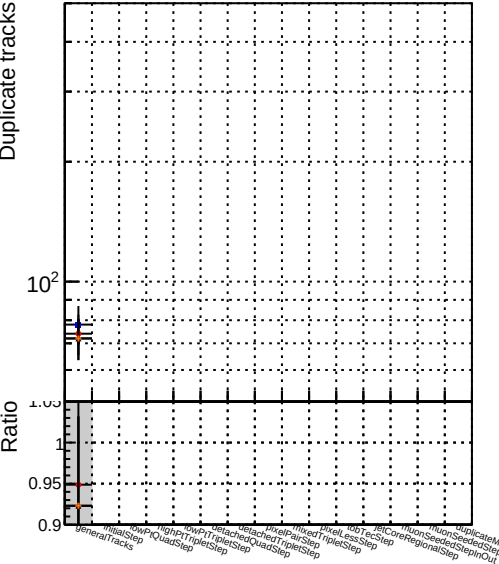
Legend: ■ DQM TT mkFit-DQM_original ■ /data2/legianni/standalone-May24/CMSSW_13_2_X_2023-06-05-1100/src/DQM TT_mkFit-DQM_updated ■ DQM TT mkFit-DQM_original_newwindows ■ DQM TT mkFit-DQM_update-mod127
