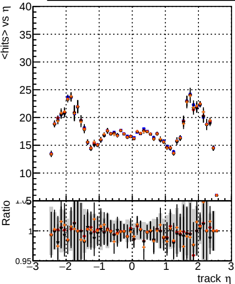
mean hits vs \eta Legend: - DQM_TT_mkFit-DQM_original (blue line) - /data2/legianni/standalone-May24/CMSSW_13_2_X_2023-06-05-1100/src/DQM_TT_mkFit-DQM_updated-0 (red line with dots) - DQM_TT_mkFit-DQM_original_newwindows (black line with dots) - DQM_TT_mkFit-DQM_update-mod127 (orange line with dots)
