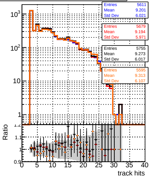
Legend: - DQM_TT_mkFit-DQM original (blue line) - /data2/legianni/standalone-May24/CMSSW_13_2_X_2023-06-05-1100/src/DQM_TT_mkFit-DQM_updated-0 (red line with error bars) - DQM_TT_mkFit-DQM original_newwindows (black line with error bars) - DQM_TT_mkFit-DQM update-mod127 (orange line)
