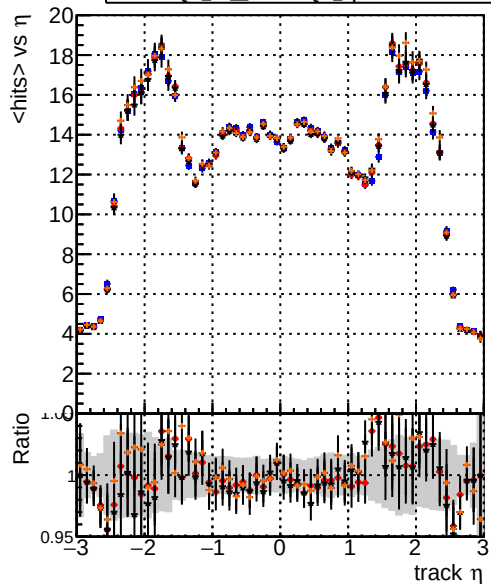
mean hits vs \eta DQM_TT_mkFit-DQM original /data2/legianni/standalone-May24/CMSSW_13_2_X_2023-06-05-1100/src/DQM_TT_mkFit-DQM_updated-0 DQM_TT_mkFit-DQM original_newwindows DQM_TT_mkFit-DQM update-mod127
