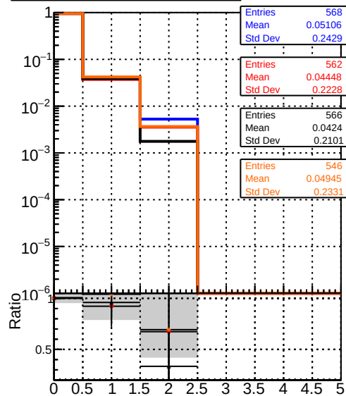
mean hits vs \eta Legend: DQM_TT_mkFit-DQM_original (blue line) /data2/legianni/standalone-May24/CMSSW_13_2_X_2023-06-05-1100/src/DQM_TT_mkFit-DQM_updated-0 (red line) DQM_TT_mkFit-DQM_original_newwindows (black line) DQM_TT_mkFit-DQM_update-mod127 (orange line)
