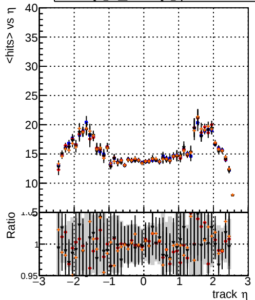
mean hits vs \eta Legend: DQM_TT_mkFit-DQM_original /data2/legianni/standalone-May24/CMSSW_13_2_X_2023-06-05-1100/src/DQM_TT_mkFit-DQM_updated-0 DQM_TT_mkFit-DQM_original_newwindows DQM_TT_mkFit-DQM_update-mod127
