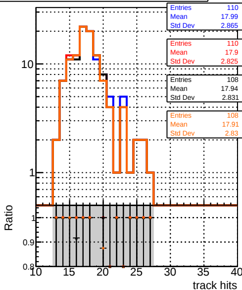
mean hit — DQM TT mkFit-DQM original — data2/legianni/standalone-May24/CMSSW_13_2_X_2023-06-05-1100/src/DQM TT_mkFit-DQM_updated40 — DQM TT_mkFit-DQM original_newwindows — DQM TT_mkFit-DQM update-mod127
