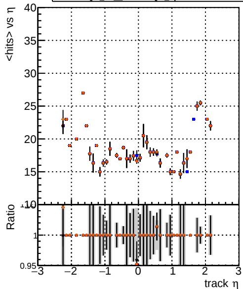
mean hit — DQM TT mkFit-DQM original — data2/legianni/standalone-May24/CMSSW_13_2_X_2023-06-05-1100/src/DQM TT_mkFit-DQM_updated40 — DQM TT_mkFit-DQM original_newwindows — DQM TT_mkFit-DQM update-mod127
