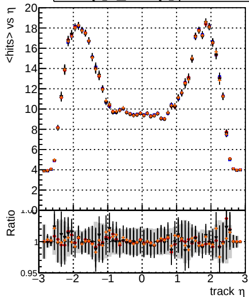
mean hits DQM_TT_mkFit-DQM_original /data2/legianni/standalone-May24/CMSSW_13_2_X_2023-06-05-1100/src/DQM_TT_mkFit-DQM_updated-0 DQM_TT_mkFit-DQM_original_newwindows DQM_TT_mkFit-DQM_update-mod127
