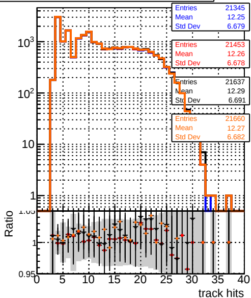
mean hits DQM_TT_mkFit-DQM_original /data2/legianni/standalone-May24/CMSSW_13_2_X_2023-06-05-1100/src/DQM_TT_mkFit-DQM_updated-0 DQM_TT_mkFit-DQM_original_newwindows DQM_TT_mkFit-DQM_update-mod127
