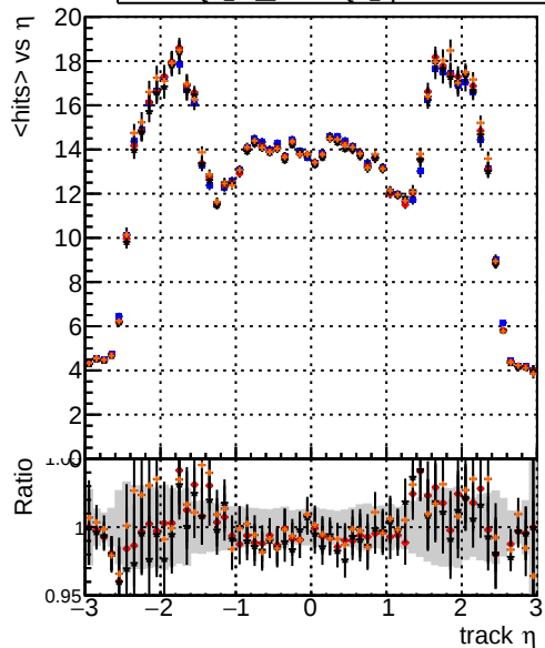
mean hit DQM_TT_mkFit-DQM_original /data2/legianni/standalone-May24/CMSSW_13_2_X_2023-06-05-1100/src/DQM_TT_mkFit-DQM_updated-0 DQM_TT_mkFit-DQM_original_newwindows DQM_TT_mkFit-DQM_update-mod127
