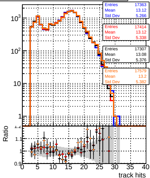
mean hit DQM_TT_mkFit-DQM_original /data2/legianni/standalone-May24/CMSSW_13_2_X_2023-06-05-1100/src/DQM_TT_mkFit-DQM_updated-0 DQM_TT_mkFit-DQM_original_newwindows DQM_TT_mkFit-DQM_update-mod127
