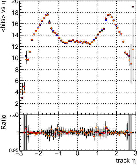
mean hits vs \eta — DQM_TT_mkFit-DQGM_original — /data2/legianni/standalone-May24/CMSSW_13_2_X_X2006-05-1100/src/DQM_TT_mkFit-DQGM_updated0 — DQM_TT_mkFit-DQGM_original_newwinds — DQM_TT_mkFit-DQGM_update-mod127
