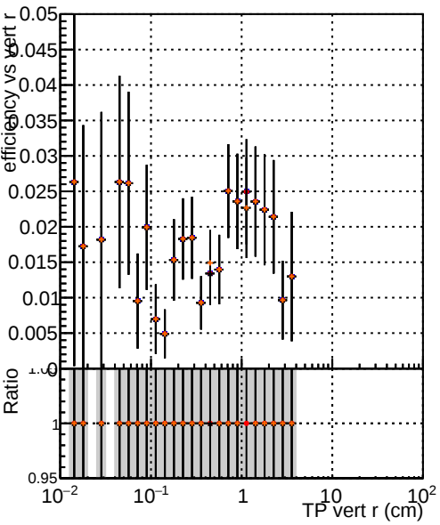
Efficiency vs vertpos Legend: DQM TT mkFit-DQM original /data2/legianni/standalone-May24/CMSSW_13_2_X_2023-06-05-1100/src/DQM TT_mkFit-DQM_updated0 DQM TT_mkFit-DQM_original_newwindows DQM TT_mkFit-DQM_update-mod127
