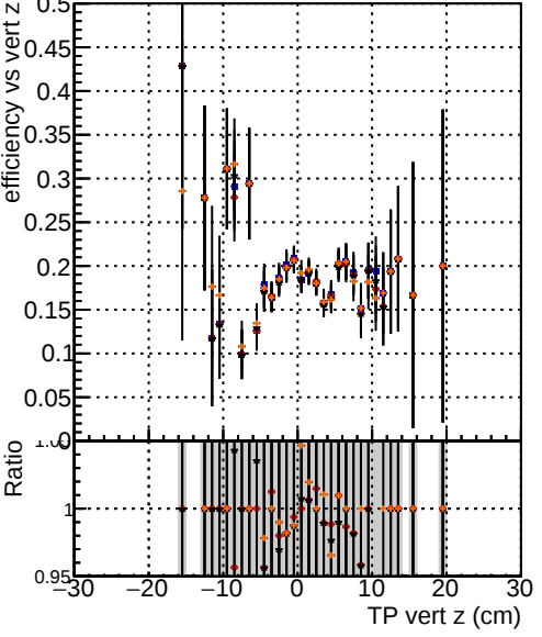
Efficiency vs vertpos Legend: — DQM TT mkFit-DQM original — /data2/legianni/standalone-May24/CMSSW_13_2_X_2023-06-05-1100/src/DQM TT_mkFit-DQM_updated0 — DQM TT_mkFit-DQM_original_newwindows — DQM TT_mkFit-DQM_update-mod127
