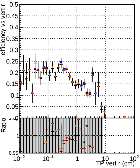
Efficiency vs vertpos Legend: — DQM TT mkFit-DQM original — /data2/legianni/standalone-May24/CMSSW_13_2_X_2023-06-05-1100/src/DQM TT_mkFit-DQM_updated0 — DQM TT_mkFit-DQM_original_newwindows — DQM TT_mkFit-DQM_update-mod127
