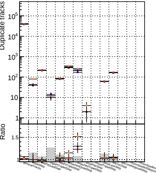
Legend: — DQM TT mkFit-DQM_original — /data2/legianni/standalone-May24/CMSSW_13_2_X_2023-06-05-1100/src/DQM_TT_mkFit-DQM_updated0 — DQM TT mkFit-DQM_original_newwindows — DQM TT mkFit-DQM_update-mod127
