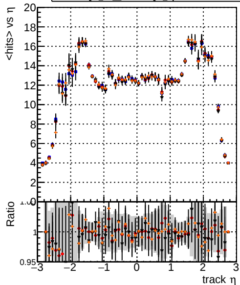
mean hits vs \eta Legend: - DQM_TT_mkFit-DQM_original (blue line) - /data2/legianni/standalone-May24/CMSSW_13_2_X_2023-06-05-1100/src/DQM_TT_mkFit-DQM_updated-0 (red line) - DQM_TT_mkFit-DQM_original_newwindows (black line) - DQM_TT_mkFit-DQM_update-mod127 (orange line)
