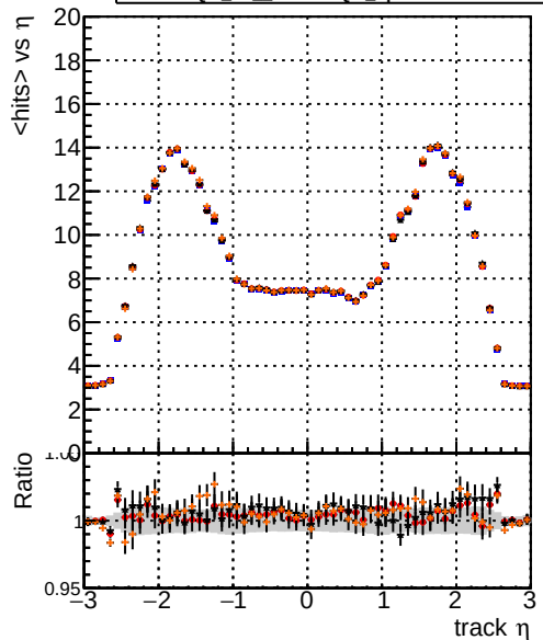
mean hits vs \eta Legend: DQM TT mkFit-DQM original, /data2/legianni/standalone-May24/CMSSW_13_2_X_2023-06-05-1100/src/DQM TT mkFit-DQM_updated0, DQM TT mkFit-DQM original_newwssos, DQM TT mkFit-DQM update-mod127
