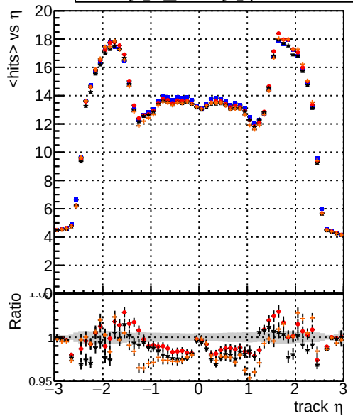
mean hits — DQM TT mkFit-DQM original — /data2/legianni/standalone-May24/CMSSW_13_2_X_2023-06-05-1100/src/DQM TT mkFit-DQM_updated-0 — DQM TT mkFit-DQM original_newwindows — DQM TT mkFit-DQM update-mod127
