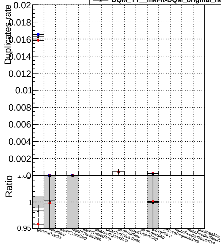
Duplicates rate vs collection Legend: DQM TT mkFit-DQM_original /data2/legianni/standalone-May24/CMSSW_13_2_X_2023-06-05-1100/src/DQM TT mkFit-DQM_updated-0 DQM TT mkFit-DQM_original_newwindows
