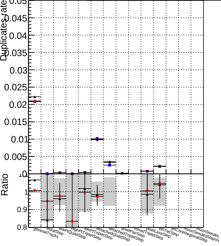
Duplicates rate vs collection Legend: DQM_TT_mkFit-DQM_original (blue square) /data2/legianni/standalone-May24/CMSSW_13_2_X_2023-06-05-1100/src/DQM_TT_mkFit-DQM_updated-0 (red circle) DQM_TT_mkFit-DQM_original_newwindows (black triangle)
