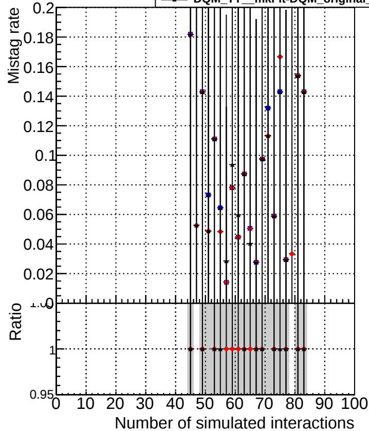
DQM_TT_mkFit-DQM_original_newwindows
