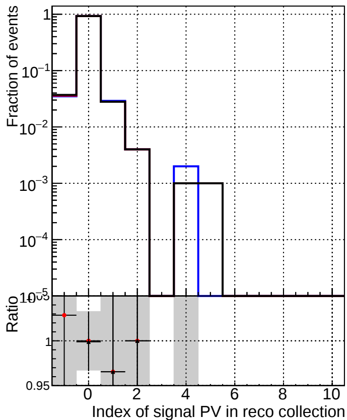
/data2/legianni/standalone-May24/CMSSW_13_2_X_2023-06-05-1100/src/DQM_TT_mkFit-DQM_updated-0
