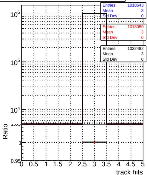
mean hits Legend: DQM_TT_mkFit-DQM_original (blue), /data2/legianni/standalone-May24/CMSSW_13_2_X_2023-06-05-1100/src/DQM_TT_mkFit-DQM_updated-0 (red), DQM_TT_mkFit-DQM_original_newwindows (black)
