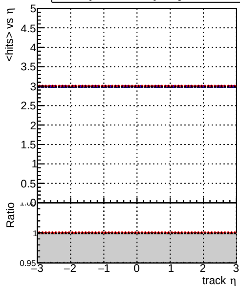
mean hits Legend: DQM_TT_mkFit-DQM_original (blue), /data2/legianni/standalone-May24/CMSSW_13_2_X_2023-06-05-1100/src/DQM_TT_mkFit-DQM_updated-0 (red), DQM_TT_mkFit-DQM_original_newwindows (black)
