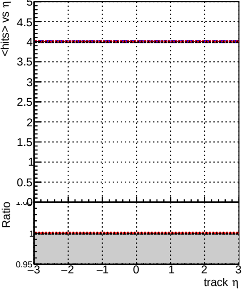
mean hits vs \eta Legend: — DQM_TT_mkFit-DQM_original (blue) — /data2/legianni/standalone-May24/CMSSW_13_2_X_2023-06-05-1100/src/DQM_TT_mkFit-DQM_updated-0 (red) — DQM_TT_mkFit-DQM_original_newwindows (black)
