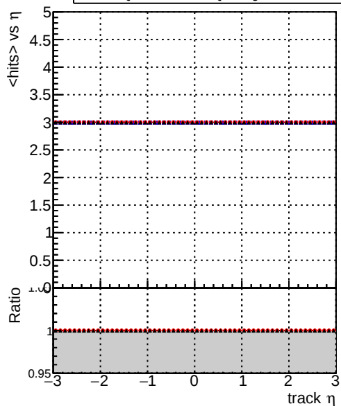
mean hits Legend: DQM_TT_mkFit-DQM_original (blue line), /data2/legianni/standalone-May24/CMSSW_13_2_X_2023-06-05-1100/src/DQM_TT_mkFit-DQM_updated-0 (red line), DQM_TT_mkFit-DQM_original_newwindows (black line)
