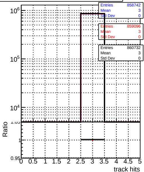
mean hits Legend: DQM_TT_mkFit-DQM_original (blue line), /data2/legianni/standalone-May24/CMSSW_13_2_X_2023-06-05-1100/src/DQM_TT_mkFit-DQM_updated-0 (red line), DQM_TT_mkFit-DQM_original_newwindows (black line)
