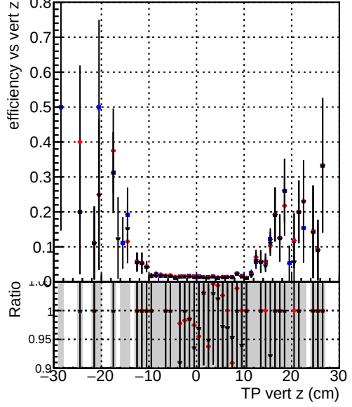
Efficiency vs vert z Legend: - DQM_TT_mkFit-DQM_original (blue circles) - /data2/legianni/standalone-May24/CMSSW_13_2_X_2023-06-05-1100/src/DQM_TT_mkFit-DQM_updated-0 (red circles) - DQM_TT_mkFit-DQM_original_newwindows (black circles)
