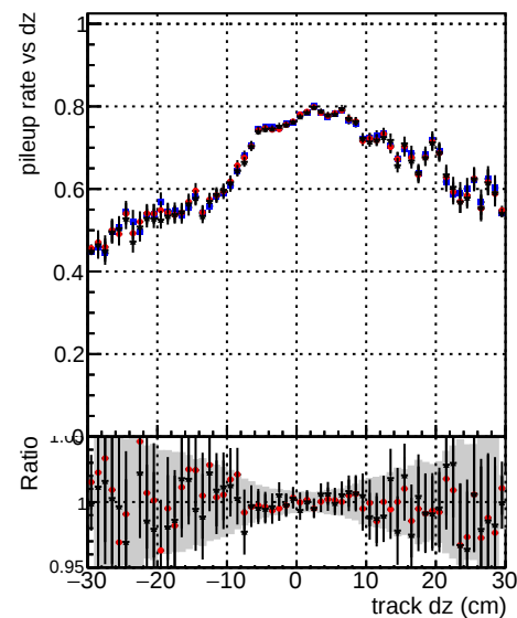
24/CMSSW_13_2_X_2023-06-05-1100/src/DQM_TT_mkFit-DQM_updated-0 newwindows
