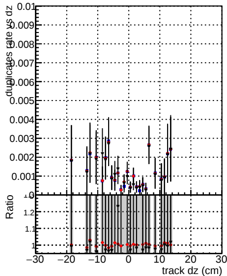
24/CMSSW_13_2_X_2023-06-05-1100/src/DQM_TT_mkFit-DQM_updated-0 newwindows
