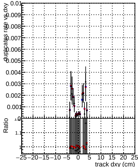
24/CMSSW_13_2_X_2023-06-05-1100/src/DQM_TT_mkFit-DQM_updated-0 newwindows
