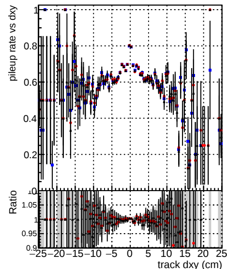
24/CMSSW_13_2_X_2023-06-05-1100/src/DQM_TT_mkFit-DQM_updated-0 newwindows
