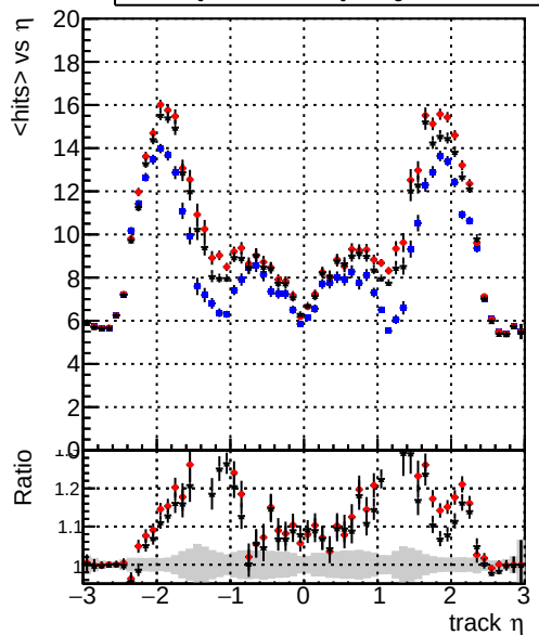
mean hits vs \eta — DQM_TT_mkFit-DQM_original — /data2/legianni/standalone-May24/CMSSW_13_2_X_2023-06-05-1100/src/DQM_TT_mkFit-DQM_updated-0 — DQM_TT_mkFit-DQM_original_newwindows
