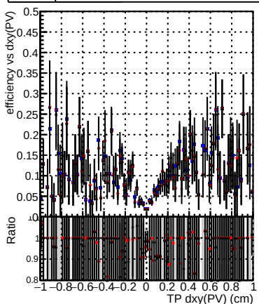
Efficiency → DQM_TT_mkFit-DQM_original_newwindows
