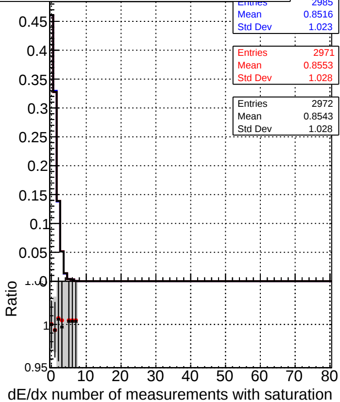
Legend for bottom row plots: DQM_TT_mkFit-DQM_original (Blue line with squares) /data2/legianni/standalone-May24/CMSSW_13_2_X_2023-06-05-1100/src/DQM_TT_mkFit-DQM_updated-0 (Red line with circles) DQM_TT_mkFit-DQM_original_newwindows (Black line with crosses)
