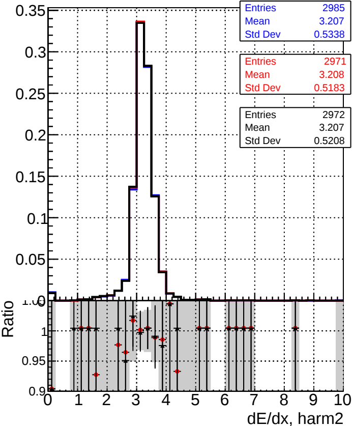
Legend for bottom row plots: DQM_TT_mkFit-DQM_original (Blue line with squares) /data2/legianni/standalone-May24/CMSSW_13_2_X_2023-06-05-1100/src/DQM_TT_mkFit-DQM_updated-0 (Red line with circles) DQM_TT_mkFit-DQM_original_newwindows (Black line with crosses)
