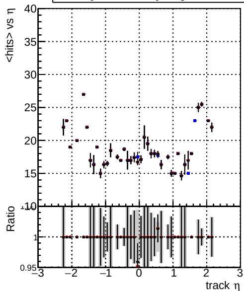
mean hits vs \eta — DQM_TT_mkFit-DQM_original — /data2/legianni/standalone-May24/CMSSW_13_2_X_2023-06-05-1100/src/DQM_TT_mkFit-DQM_updated-0 — DQM_TT_mkFit-DQM_original_newwindows
