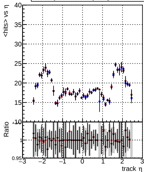
mean hits — DQM_TT_mkFit-DQM_original — /data2/legianni/standalone-May24/CMSSW_13_2_X_2023-06-05-1100/src/DQM_TT_mkFit-DQM_updated-0 — DQM_TT_mkFit-DQM_original_newwindows
