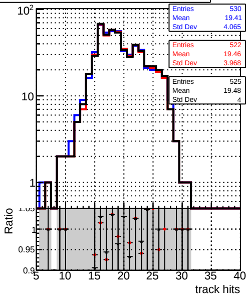
mean hits — DQM_TT_mkFit-DQM_original — /data2/legianni/standalone-May24/CMSSW_13_2_X_2023-06-05-1100/src/DQM_TT_mkFit-DQM_updated-0 — DQM_TT_mkFit-DQM_original_newwindows
