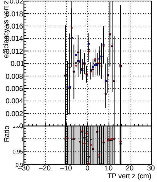
Efficiency vs vert z Legend: \bullet DQM_TT_mkFit-DQM_original \bullet /data2/legianni/standalone-May24/CMSSW_13_2_X_2023-06-05-1100/src/DQM_TT_mkFit-DQM_updated-0 \bullet DQM_TT_mkFit-DQM_original_newwindows
