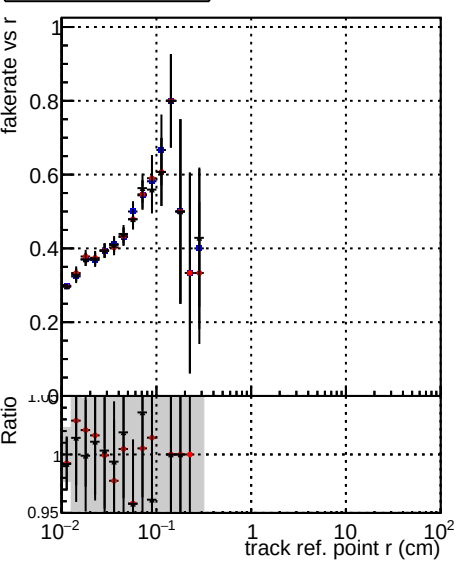
Legend: DQM TT mkFit-DQM original (blue squares), /data2/legianni/standalone-May24/CMSSW_13_2_X_2023-06-05-1100/src/DQM TT_mkFit-DQM_updated-0 (red circles), DQM TT_mkFit-DQM original newwindows (black crosses)
