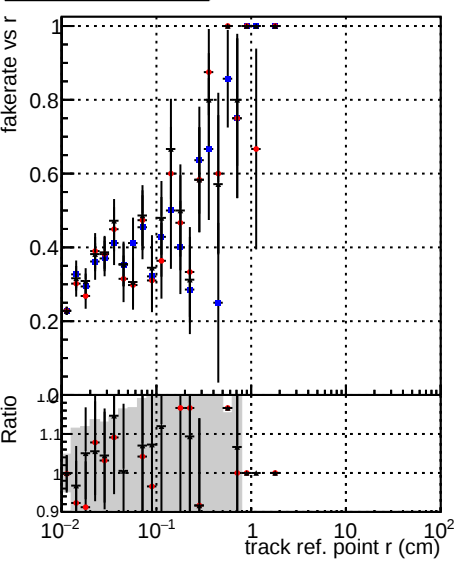
Legend: DQM TT mkFit-DQM original (black squares), /data2/legianni/standalone-May24/CMSSW_13_2_X_2023-06-05-1100/src/DQM_TT_mkFit-DQM_updated-0 (red circles), DQM_TT_mkFit-DQM original newwindows (blue circles)
