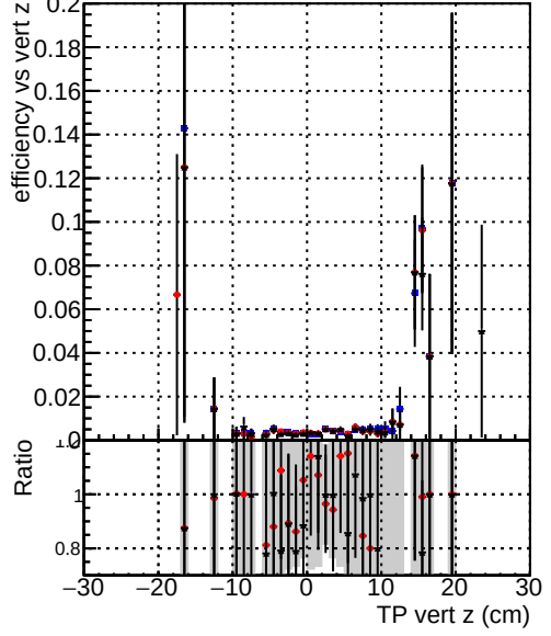
Efficiency vs. TP vert z Legend: DQM TT mkFit-DQM_original (blue circles) /data2/legianni/standalone-May24/CMSSW_13_2_X_2023-06-05-1100/src/DQM TT mkFit-DQM_updated-0 (red circles) DQM TT mkFit-DQM_original_newwindows (black circles)
