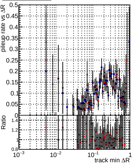
Legend: DQM TT mkFit-DQM original (blue dots), /data2/legianni/standalone-May24/CMSSW_13_2_X_2023-06-05-1100/src/DQM_TT_mkFit-DQM_updated-0 (red dots), DQM TT mkFit-DQM original newwindows (black dots)
