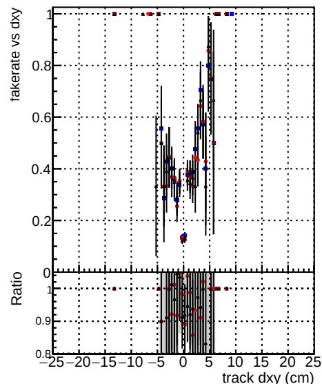
DOM TT mkFit-DQM original /data2/legiann/standalone-May24/CMSW_13_2_X_2023-06-05-1100/src/DQM_TT_mkFit-DQM_updated-0 DOM TT mkFit-DQM original newwindows
