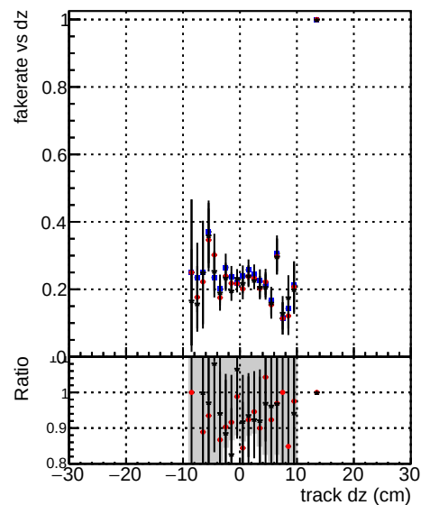
DOM TT mkFit-DQM original /data2/legiann/standalone-May24/CMSW_13_2_X_2023-06-05-1100/src/DQM_TT_mkFit-DQM_updated-0 DOM TT mkFit-DQM original newwindows
