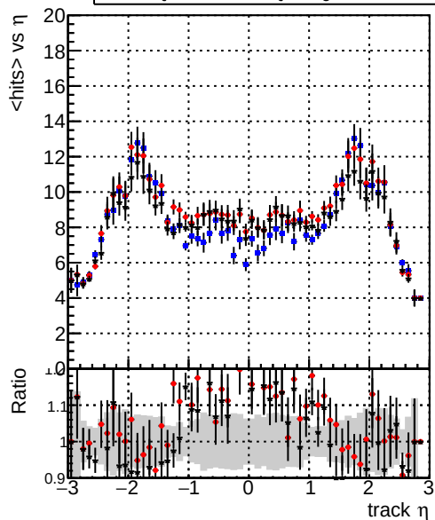
mean hit — DQM_TT_mkFit-DQM_original — /data2/legianni/standalone-May24/CMSSW_13_2_X_2023-06-05-1100/src/DQM_TT_mkFit-DQM_updated-0 — DQM_TT_mkFit-DQM_original_newwindows
