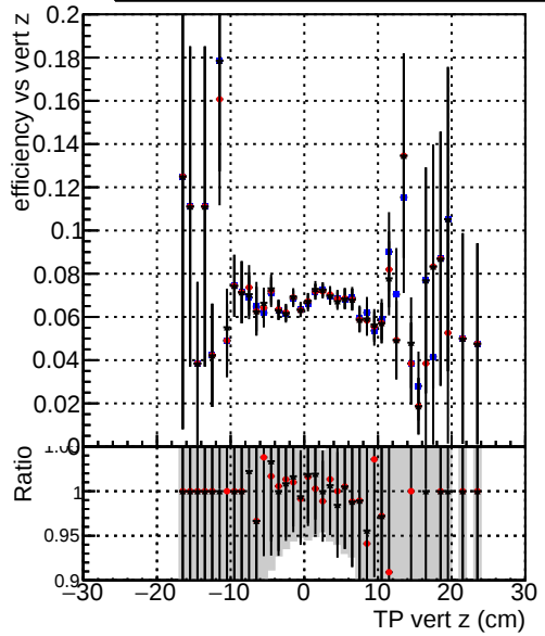
Efficiency vs. sim PV z —●— DQM_TT_mkFit-DQM_original —●— /data2/legianni/standalone-May24/CMSSW_13_2_X_2023-06-05-1100/src/DQM_TT_mkFit-DQM_updated-0 —●— DQM_TT_mkFit-DQM_original_newwindows
