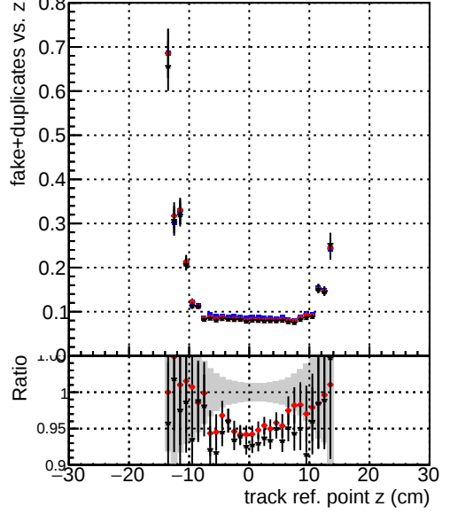
—●— DQM_TT_mkFit-DQM_original —●— /data2/legianni/standalone-May24/CMSSW_13_2_X_2023-06-05-1100/src/DQM_TT_mkFit-DQM_updated-0 —●— DQM_TT_mkFit-DQM_original_newwindows
