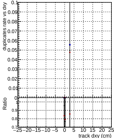
24/CMSSW_13 newwindows
