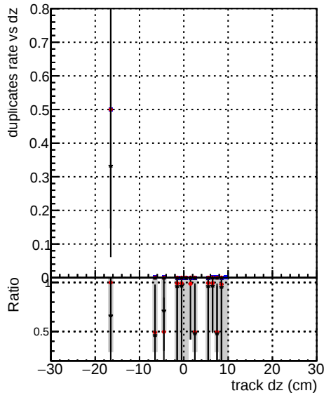
24/CMSSW_13 newwindows
