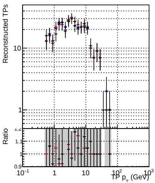
Legend: - DQM_TT_mkFit-DQM_original (blue stars) - /data2/legianni/standalone-May24/CMSSW_13_2_X_2023-06-05-1100/src/DQM_TT_mkFit-DQM_updated-0 (red stars) - DQM_TT_mkFit-DQM_original_newwindows (black stars)
