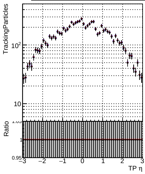
Legend: - DQM_TT_mkFit-DQM_original (blue stars) - /data2/legianni/standalone-May24/CMSSW_13_2_X_2023-06-05-1100/src/DQM_TT_mkFit-DQM_updated-0 (red stars) - DQM_TT_mkFit-DQM_original_newwindows (black stars)
