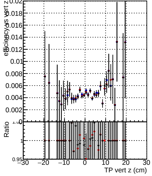
Efficiency vs vert z Legend: DQM_TT_mkFit-DQM_original (blue stars) /data2/legianni/standalone-May24/CMSSW_13_2_X_2023-06-05-1100/src/DQM_TT_mkFit-DQM_updated-0 (red stars) DQM_TT_mkFit-DQM_original_newwindows (black stars)
