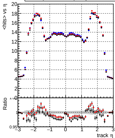
mean hits — DQM_TT_mkFit-DQM_original — /data2/legianni/standalone-May24/CMSSW_13_2_X_2023-06-05-1100/src/DQM_TT_mkFit-DQM_updated-0 — DQM_TT_mkFit-DQM_original_newwindows
