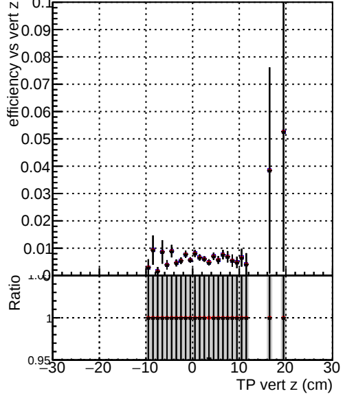
Efficiency vs. TP vert z Legend: DQM_TT_mkFit-DQM_original /data2/legianni/standalone-May24/CMSSW_13_2_X_2023-06-05-1100/src/DQM_TT_mkFit-DQM_updated-0 DQM_TT_mkFit-DQM_original_newwindows
