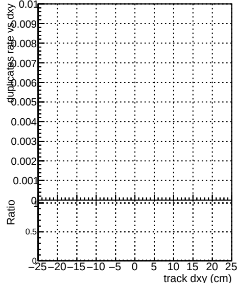
24/CMSSW_13 _newwindows
