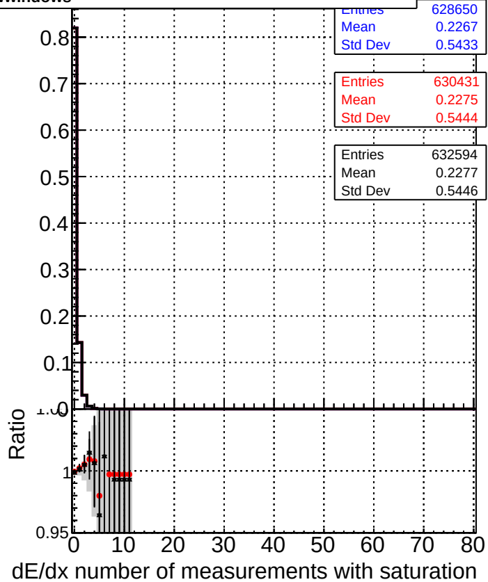
/data2/legianni/standalone-May24/CMSSW_13_2_X_2023-06-05-1100/src/DQM_TT_mkFit-DQM_updated-0
