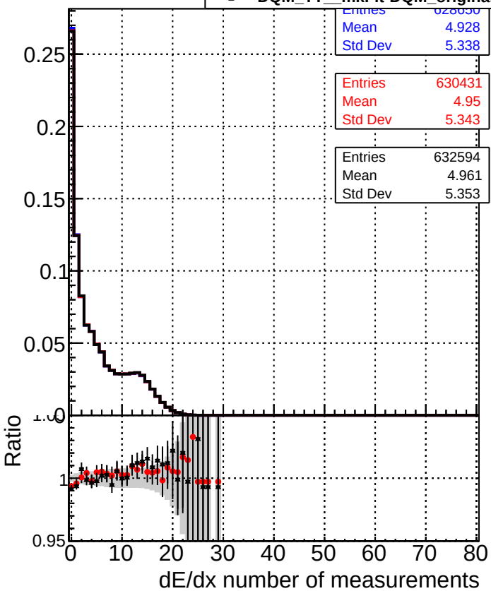
DQM_TT_mkFit-DQM_original_newwindows
