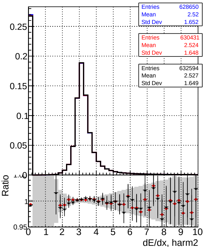
DQM_TT_mkFit-DQM_original
