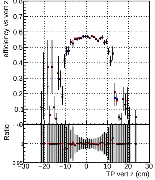
Efficiency vs. TP vert z (cm) — + DQM_TT_mkFit-DQM_original — + /data2/legianni/standalone-May24/CMSSW_13_2_X_2023-06-05-1100/src/DQM_TT_mkFit-DQM_updated-0 — + DQM_TT_mkFit-DQM_original_newwindows
